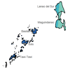
RX5day
